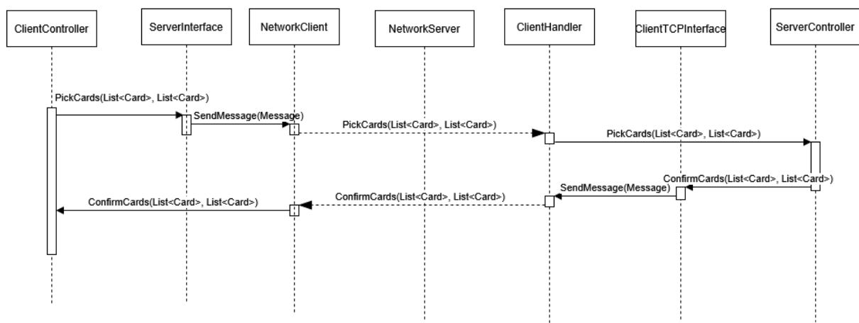
Card Pick TCP sequence diagram
