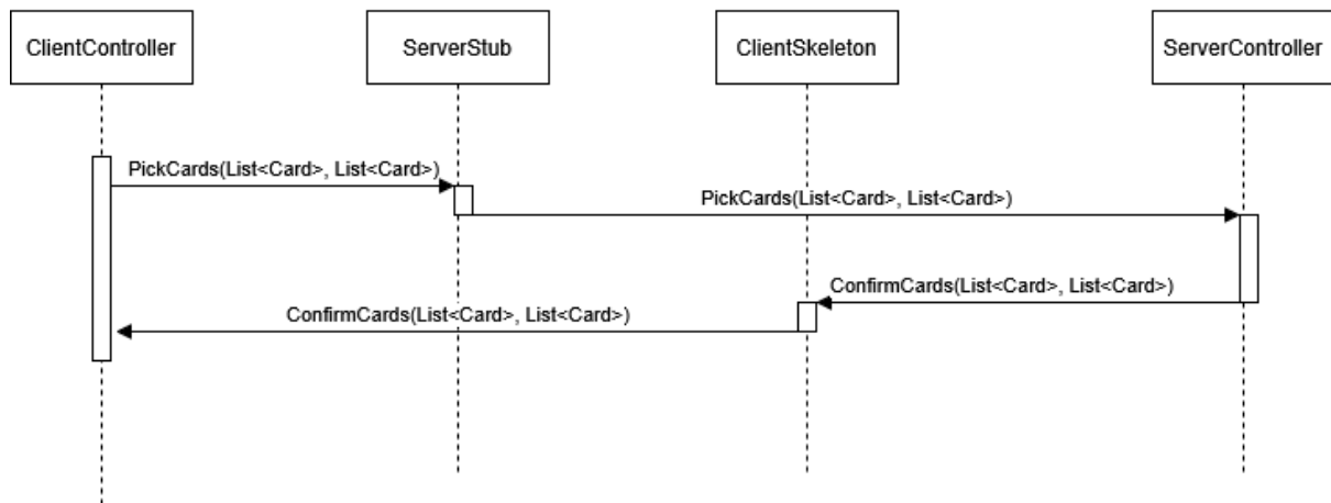
Card Pick RMI sequence diagram
